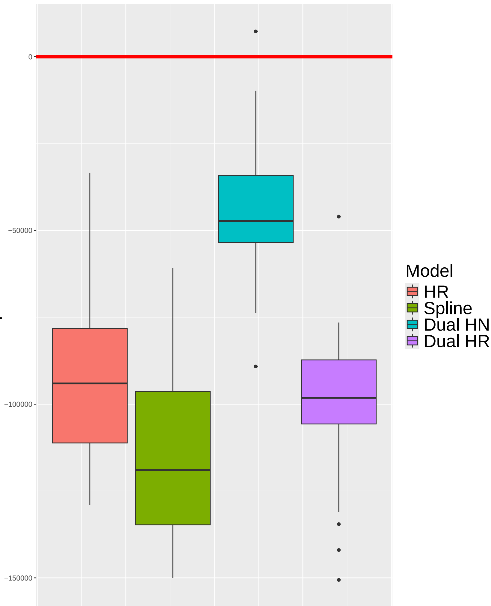
Integrated Squared Error on mean log lambda
